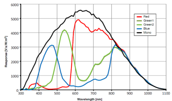
MV-CA050-20GM/GC Quantum Efficiency
