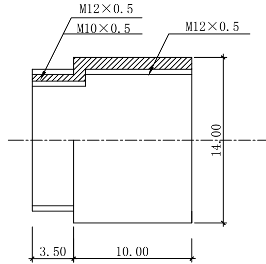
S-mount Tube ST10
