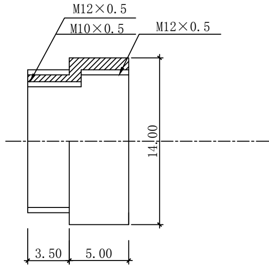
S-mount tube ST05
