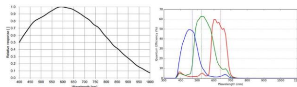
MV-CA016-10UM/UC
