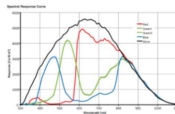
MV-CA020-20GC Quantum Efficiency
